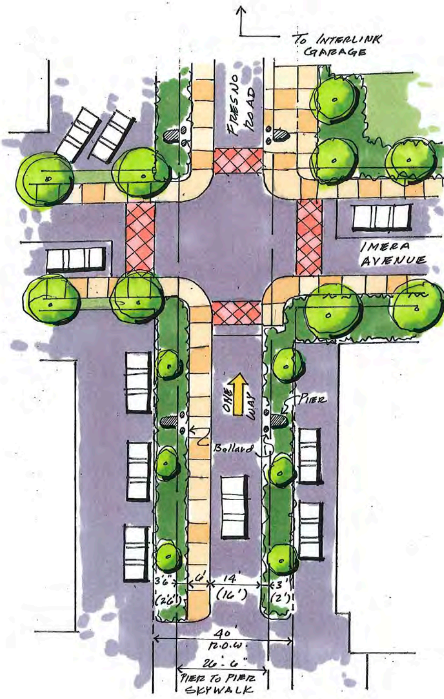
14' and 16' Wide One Way Roadway Layout
