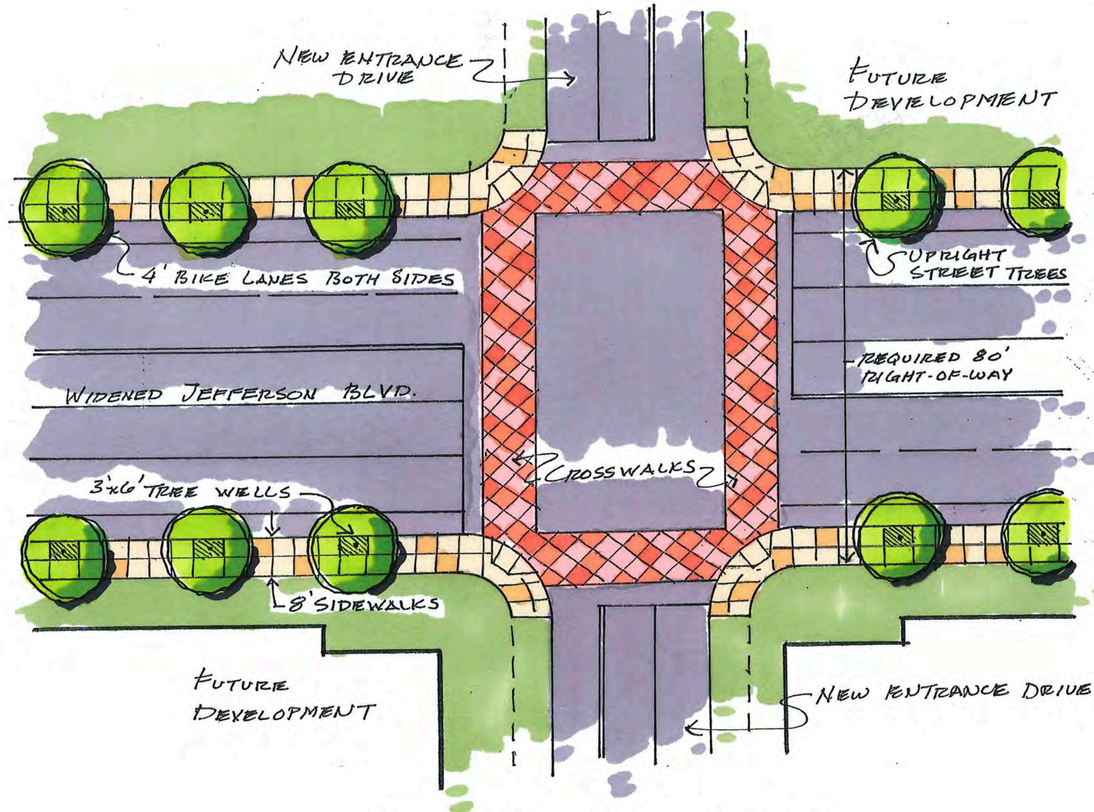
Plan: Typical Streetscape South of Interlink in Vicinity of Future Development Entrance Drives
