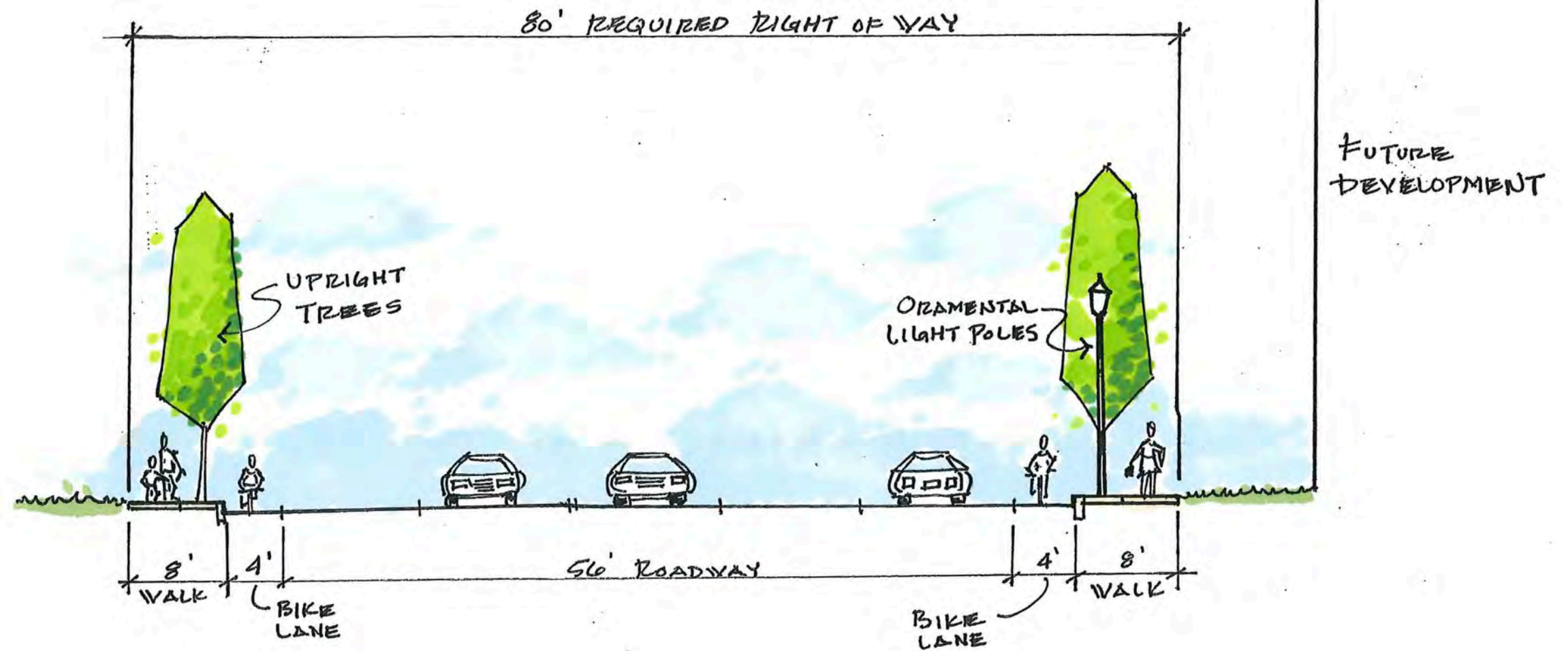
Section: Typical Streetscape South of Interlink
